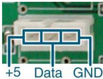
Figure 13: 1-Wire Pinout
