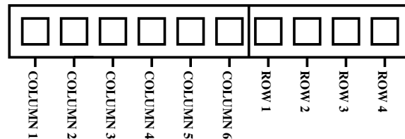
Figure 15: Keypad Connector
