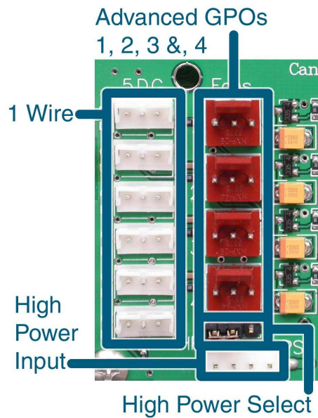
Figure 10: Pin Connectors
