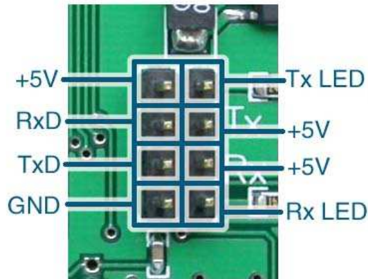
Figure 8: Rx /Tx LED Header
