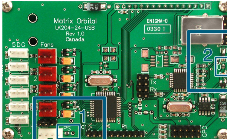
Figure 3: Jumper Locations
