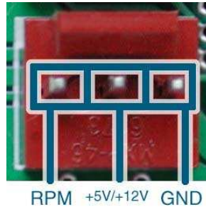
Figure 9: Fan Headers
