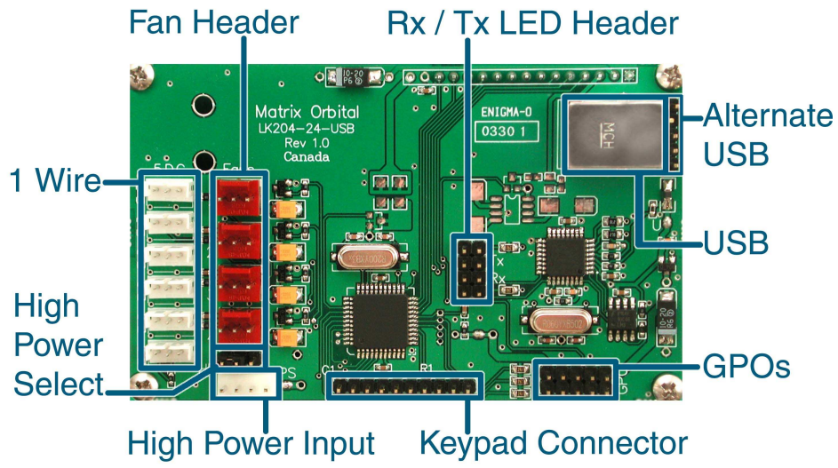
Figure 2: Electrical Connections
