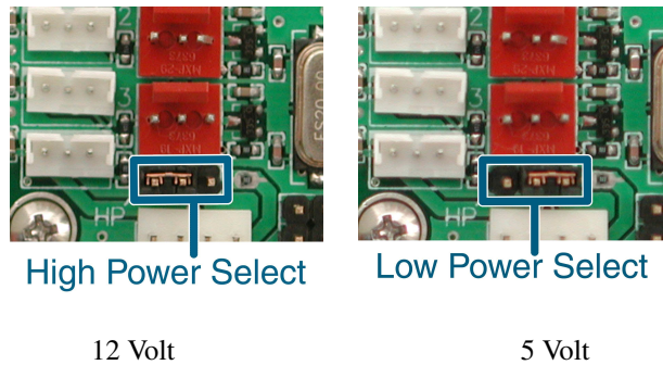
Figure 11: High / Low Power Select
