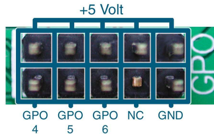
Figure 12: General Purpose Outputs
