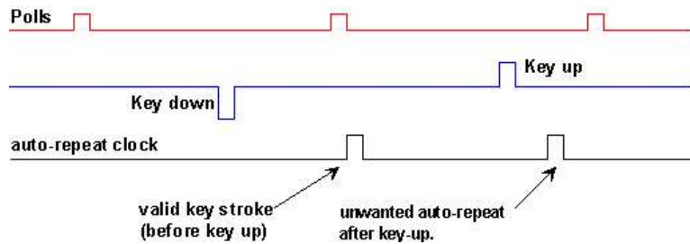
Figure 16: Poll Timing
