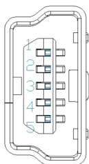
Figure 14: Mass Storage USB Connector
