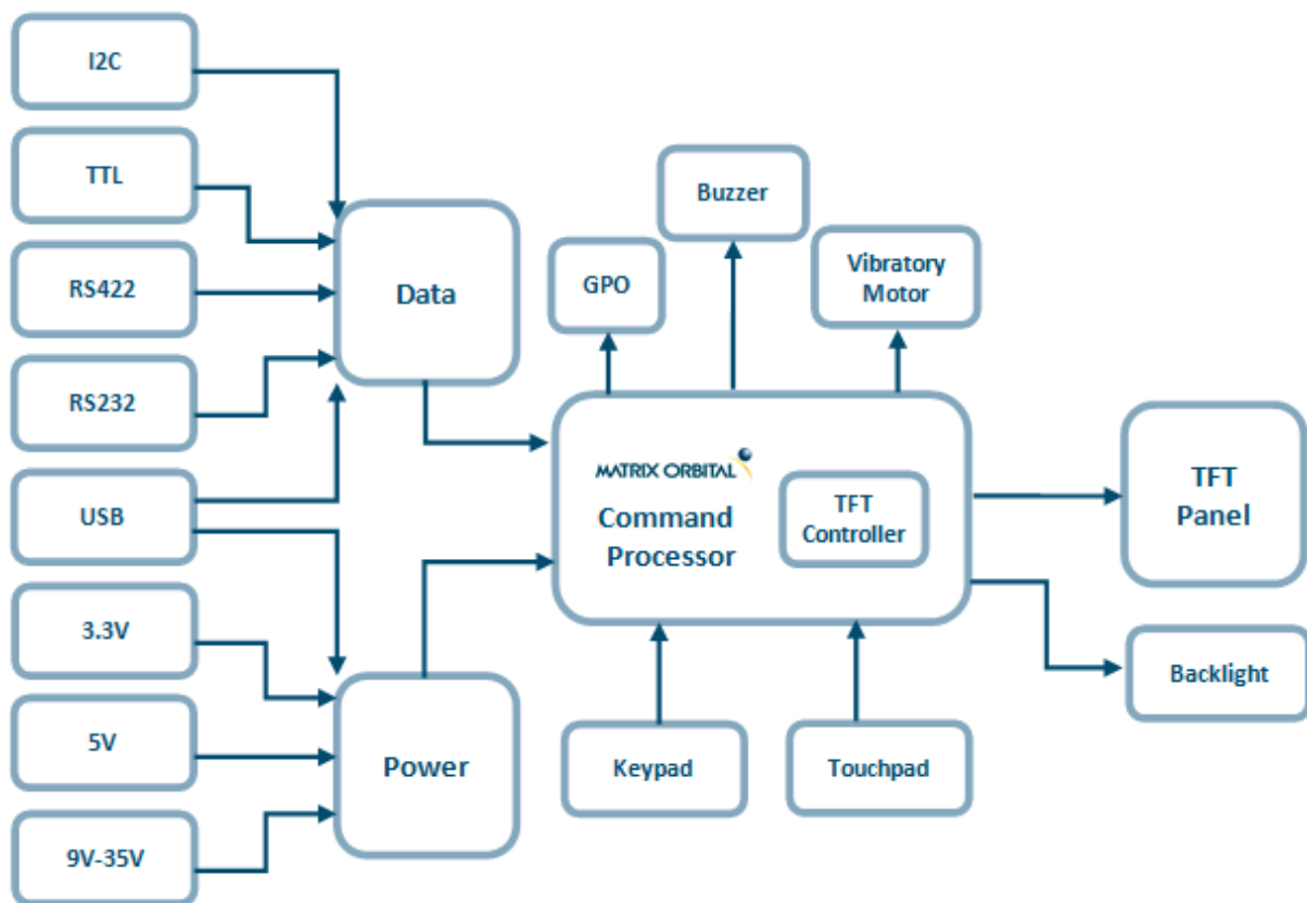
Figure 2: Functional Diagram
